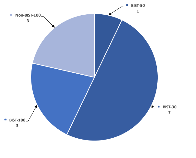
Model portfolio index distribution
